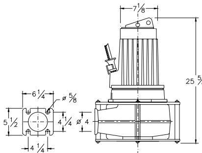
Fig. 1 Basic version Installation V
