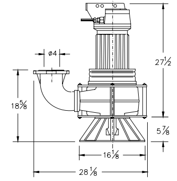
Fig. 2 Version K/P Installation T
