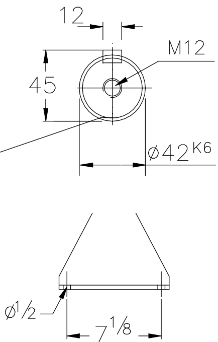
Shaft detail (in mm)
